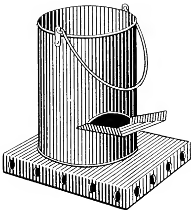
FIG. 12.—A charcoal fire pot.
